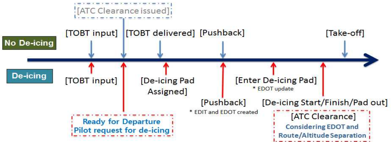
<Figure 2-14. De-icing/Anti-icing Operation Flow Diagram>
